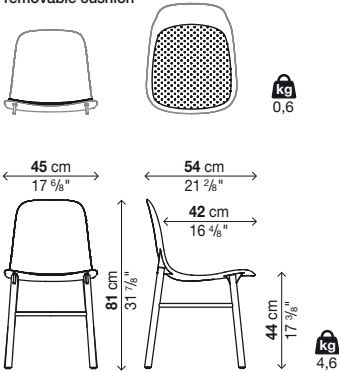
removable cushion
